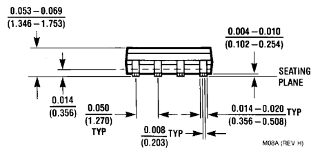
Molded Package, Small Outline, 0.15 Wide, 8-Lead (M8) Order Number NM93CS06M8, NM93CS46M8 or NM93CS56M8 NS Package Number M08A
