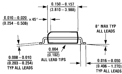
Molded Package, Small Outline, 0.15 Wide, 8-Lead (M8) Order Number NM93CS06M8, NM93CS46M8 or NM93CS56M8 NS Package Number M08A
