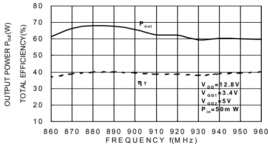
OUTPUT POWER, TOTAL EFFICIENCY, versus FREQUENCY
